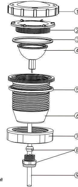
Figure 3 – Repair Parts Illustration for Plastic Spa Light
